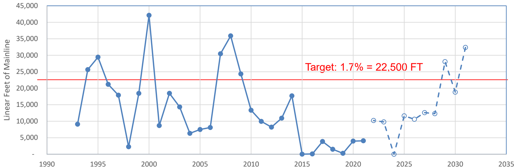
Annual Waterline Replacement (Past and Future)
